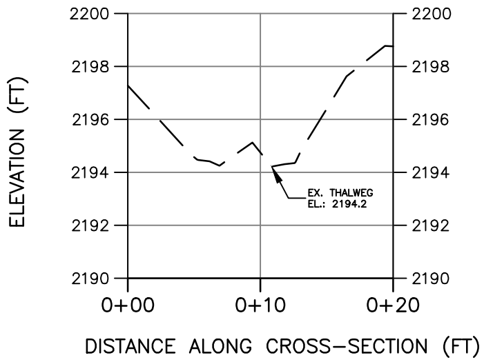
S-F21 BASELINE CROSS-SECTION A
