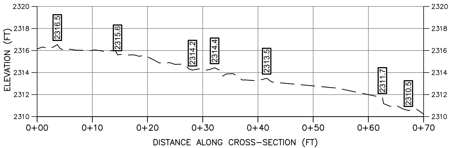
S-147 BASELINE THALWEG PROFILE
