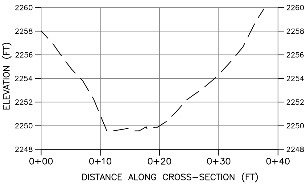
S-IJ60 BASELINE CROSS-SECTION A RIFFLE
