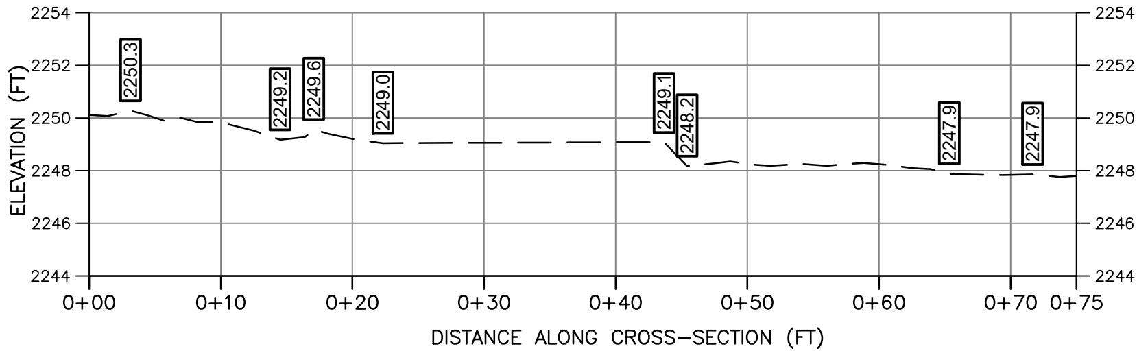
S-IJ60 BASELINE THALWEG PROFILE
