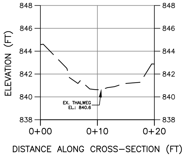
S-VV13B BASELINE CROSS-SECTION B DOWNSTREAM FROM CULVERT OUTLET (POOL)
