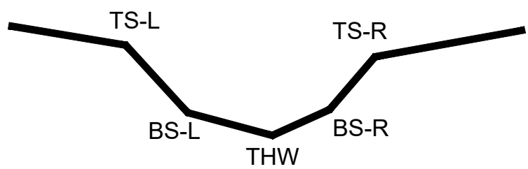
TYPICAL 5-POINT CROSS-SECTION (FACING DOWNSTREAM)
