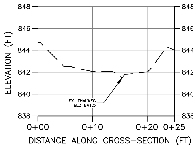
S-VV13B BASELINE CROSS-SECTION A UPSTREAM FROM CULVERT INLET (RIFFLE)
