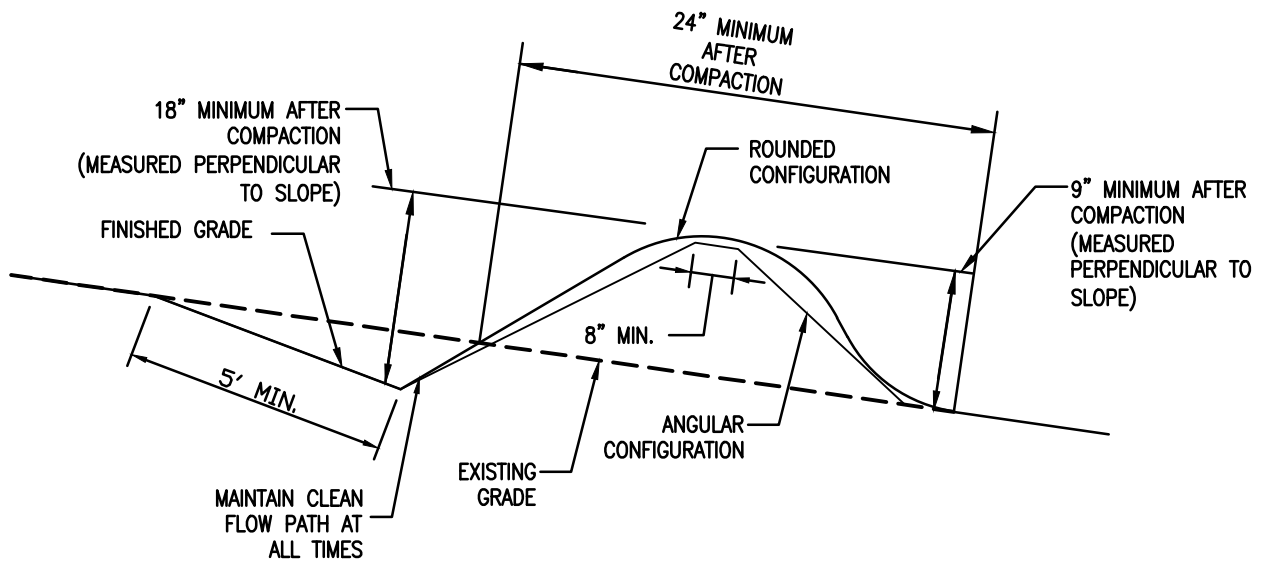
SECTION A-A (TEMPORARY INSTALLATION)
