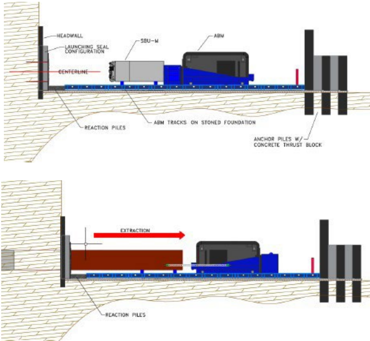
Figure 1. Appalachian National Scenic Trail Crossing – Manned Tunnel Bore Typical Drawings
