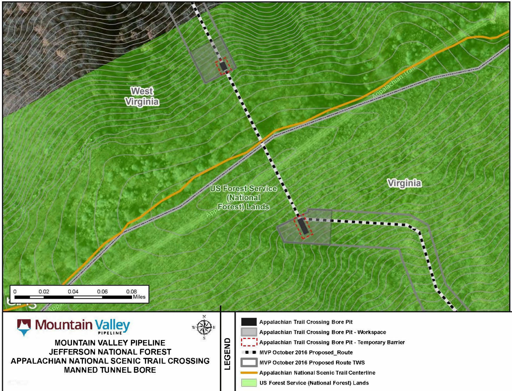
Figure 2. Appalachian National Scenic Trail Crossing – Manned Tunnel Bore
