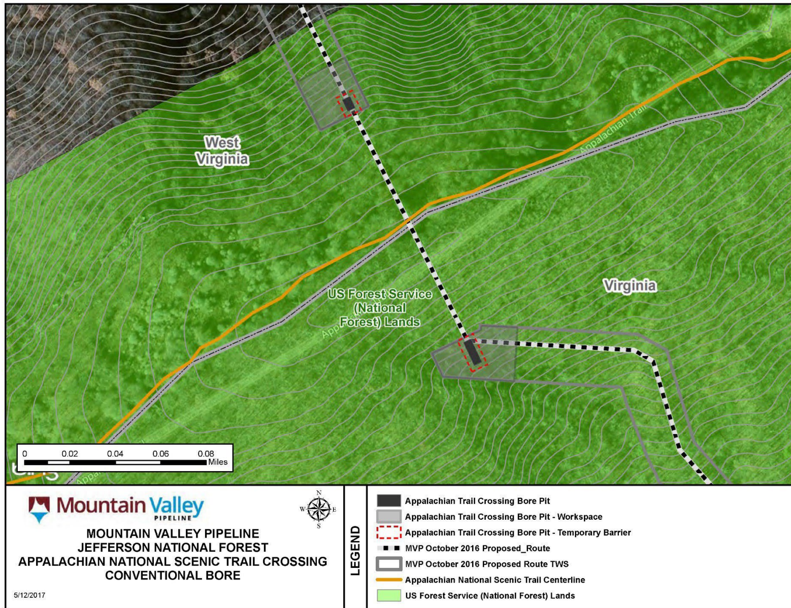
Figure 8. Appalachian National Scenic Trail Crossing – Conventional Bore
