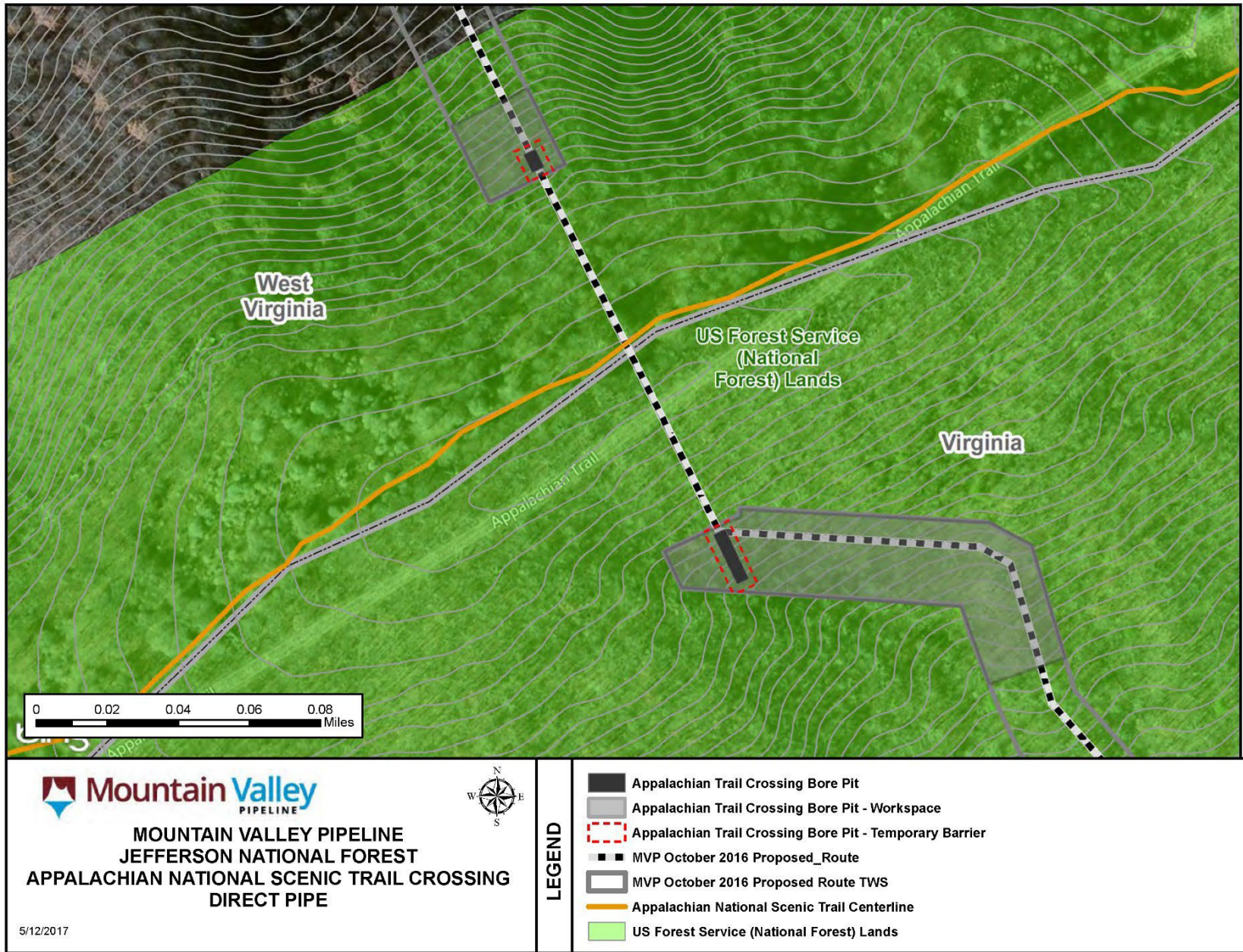
Figure 6. Appalachian National Scenic Trail Crossing – Direct Pipe
