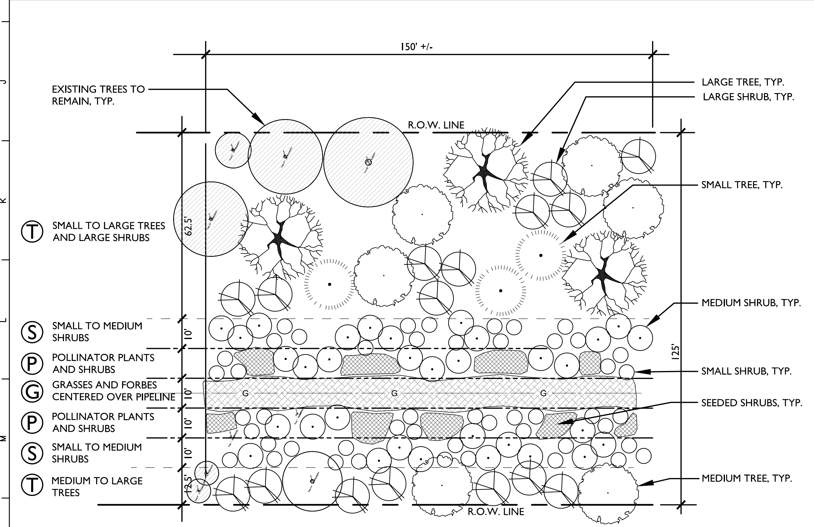
3 Typical Planting Plan - Zone 4 - High Ridge and Bedrock Outcrops 1" = 20' SCALE: 1" = 20'
