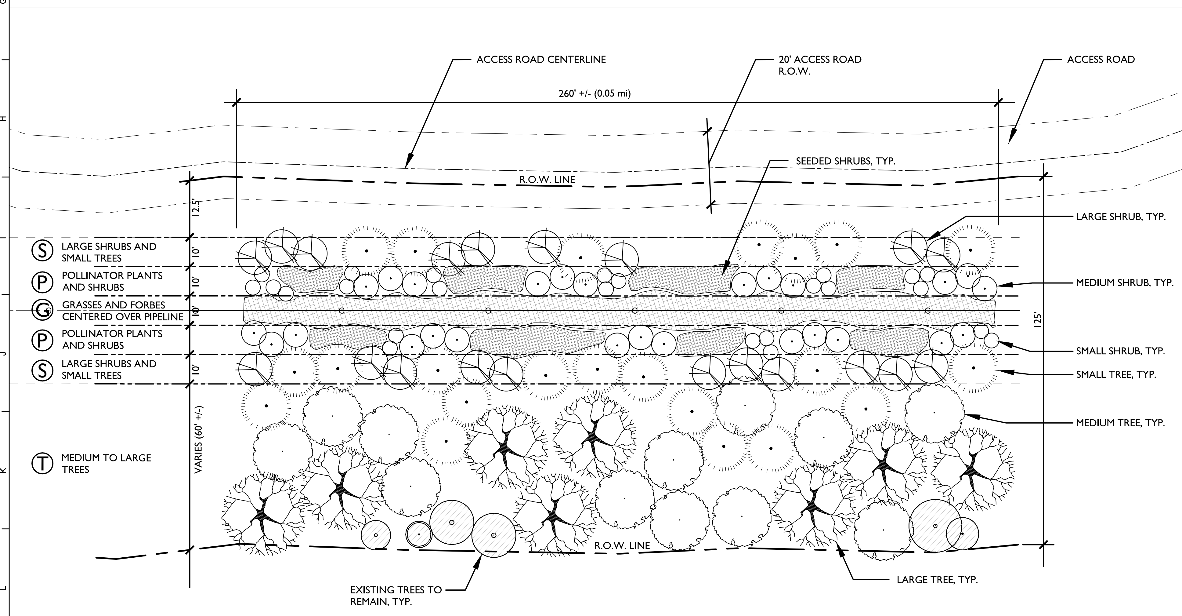
2 Typical Planting Plan - Zone 6 - Dry, Stony or Cobble Adjoining the Access Road (Moderate Slopes) 1" = 20'
